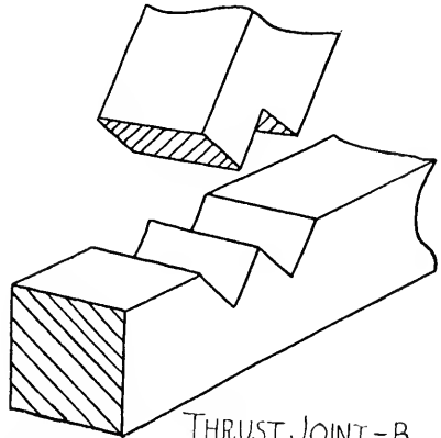
THRUST JOINT-B
